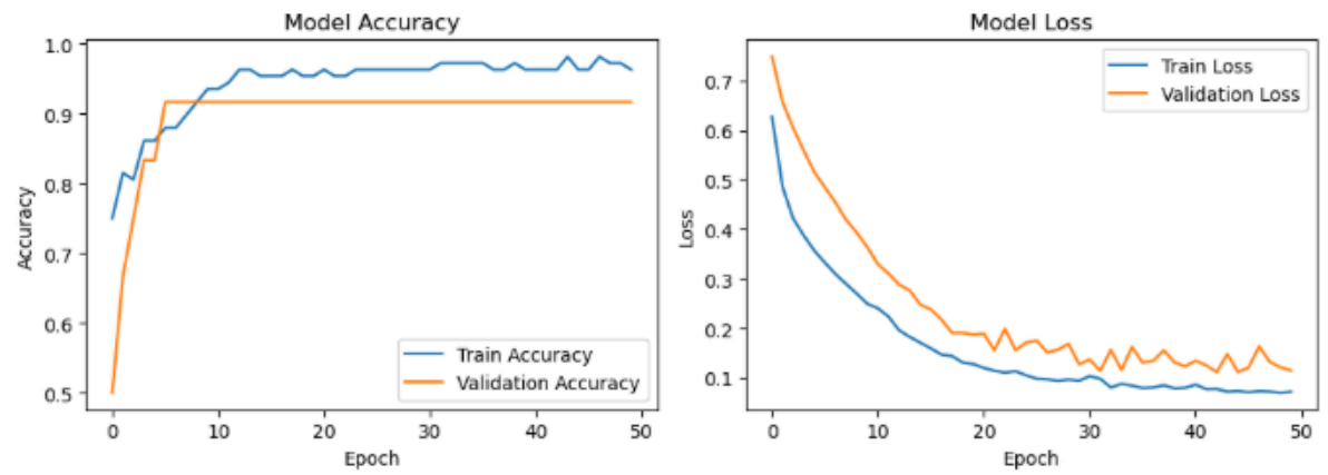
Hidden Layers: [32, 16, 8] | Activation: tanh
