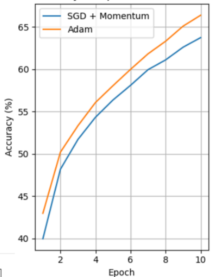
Accuracy Comparison on CIFAR-10
