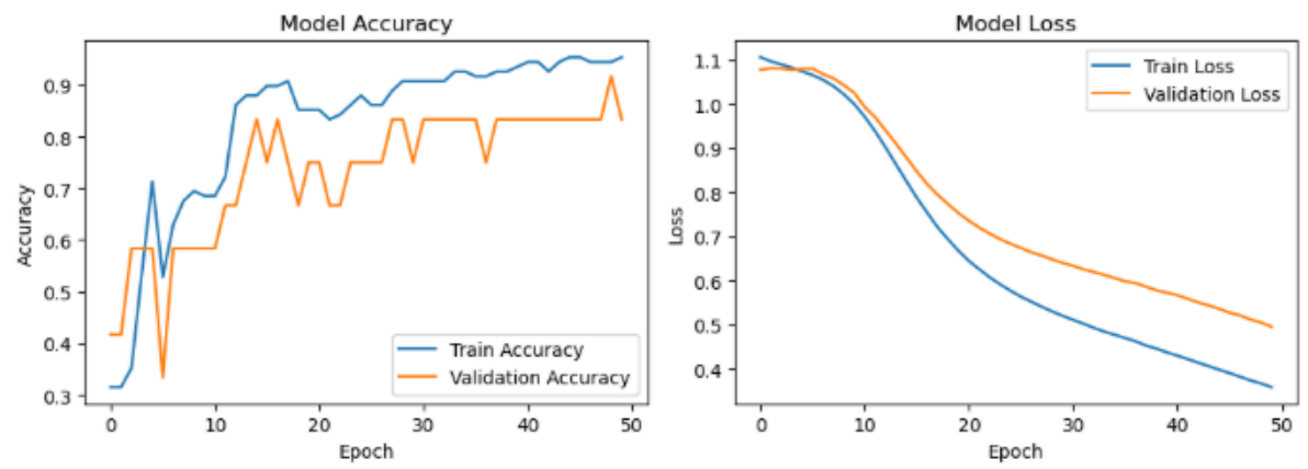
Hidden Layers: [32, 16, 8] | Activation: sigmoid
